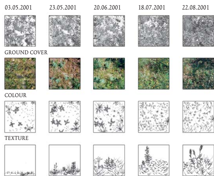
Figure 2 Aesthetic view on a spontaneous growing stand (1 x 1 m²) (Agropyretea-intermedio-repentis community) (Abicht 2001, modified)
