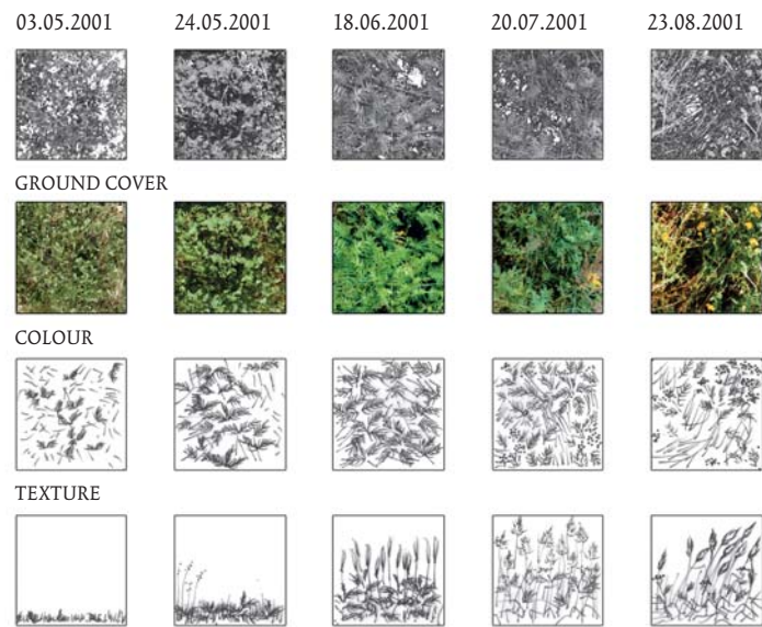
Figure 1 Aesthetic view on a spontaneous growing stand (1 x 1 m²) (Artemisio-Tanacetetum) (Abicht 2001, modified)
